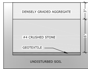
FIGURE 1. DETAIL
